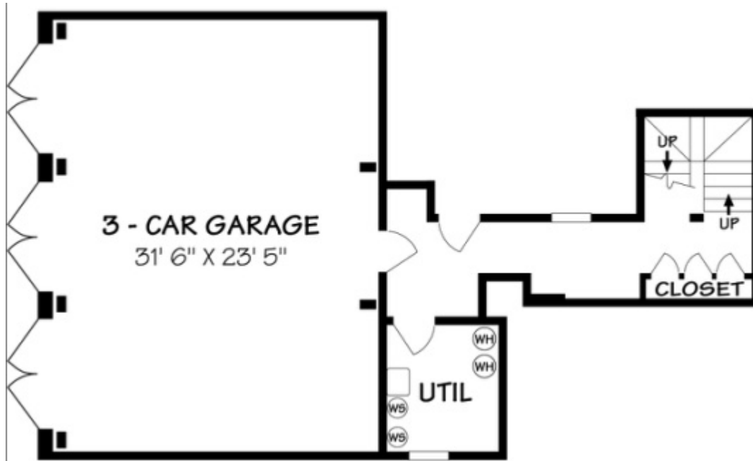
LOWER LEVEL
